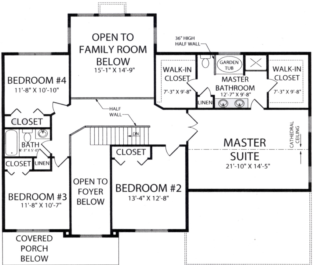
SYDNEY SECOND FLOOR PLAN
